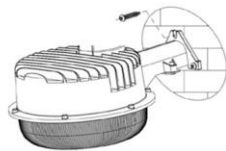
Direct Mounting
