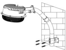
Arm Mounting
